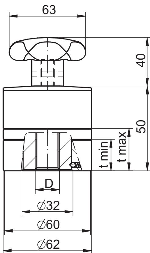
Power clamping nut ESBS with stargrip
