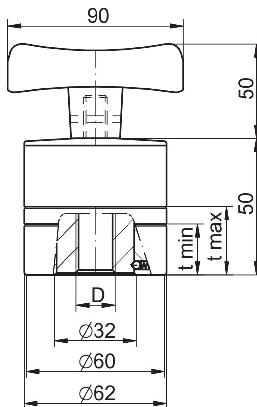
Power clamping nut ESBT with T-grip
